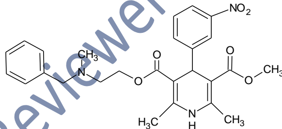
Figure 2: Chemical structure of Nicardipine
