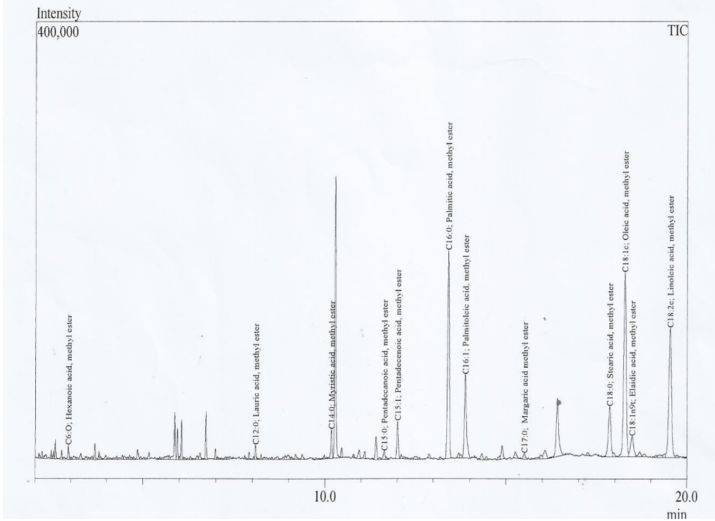
Fig 4: Graphical representation of GC-MS analysis of sample 4
