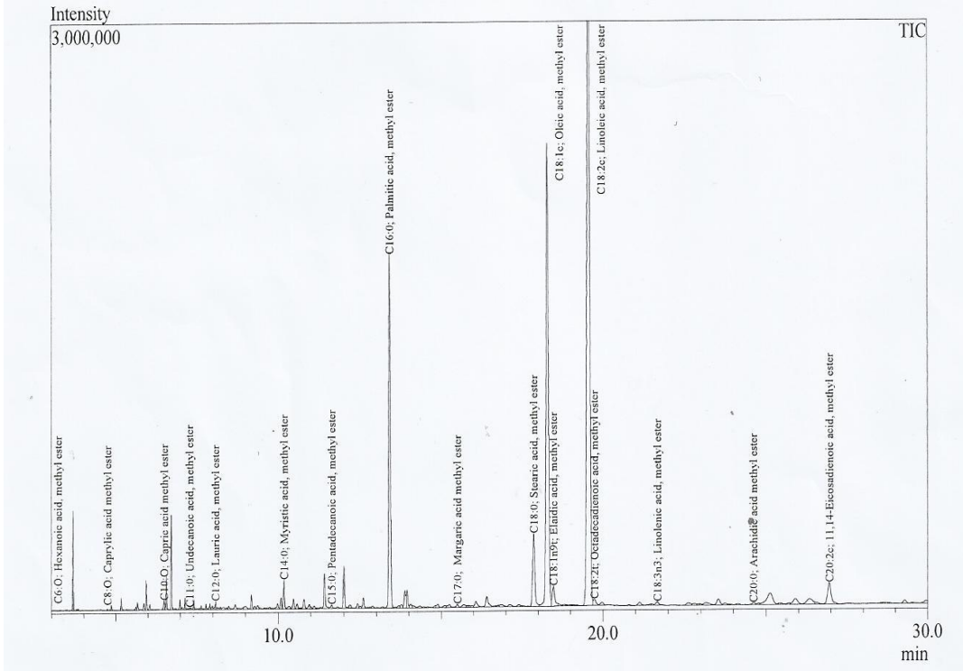
Fig 3: Graphical representation of GC-MS analysis of sample 3
