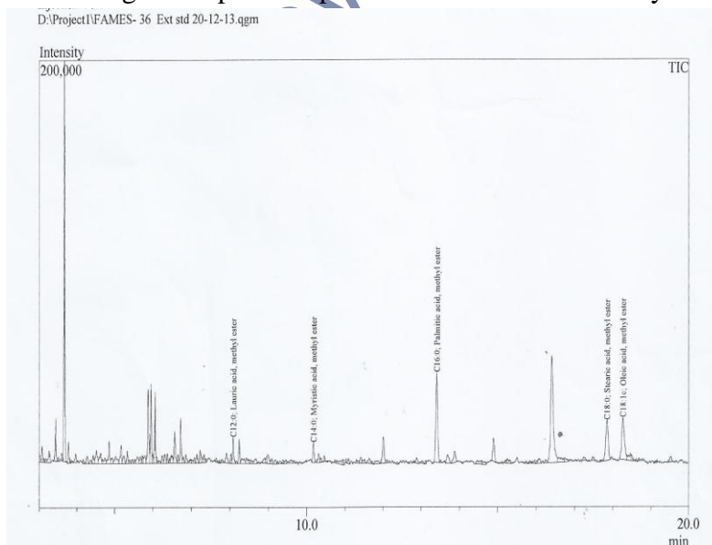
Fig 2: Graphical representation of GC-MS analysis of sample 2
