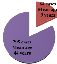
Fig 2: Age distribution of CNS tumors
