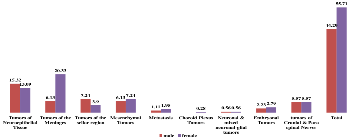
Fig. 6: Sex distribution of CNS tumors in percentage
