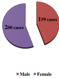
Fig. 1: Sex distribution of CNS tumors
