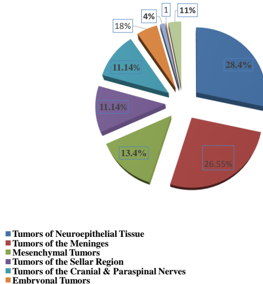
Fig. 5: Frequency of CNS tumors in 359 cases
