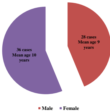
Fig.3: Pediatric age distribution in relation to sex n= 64 patients
