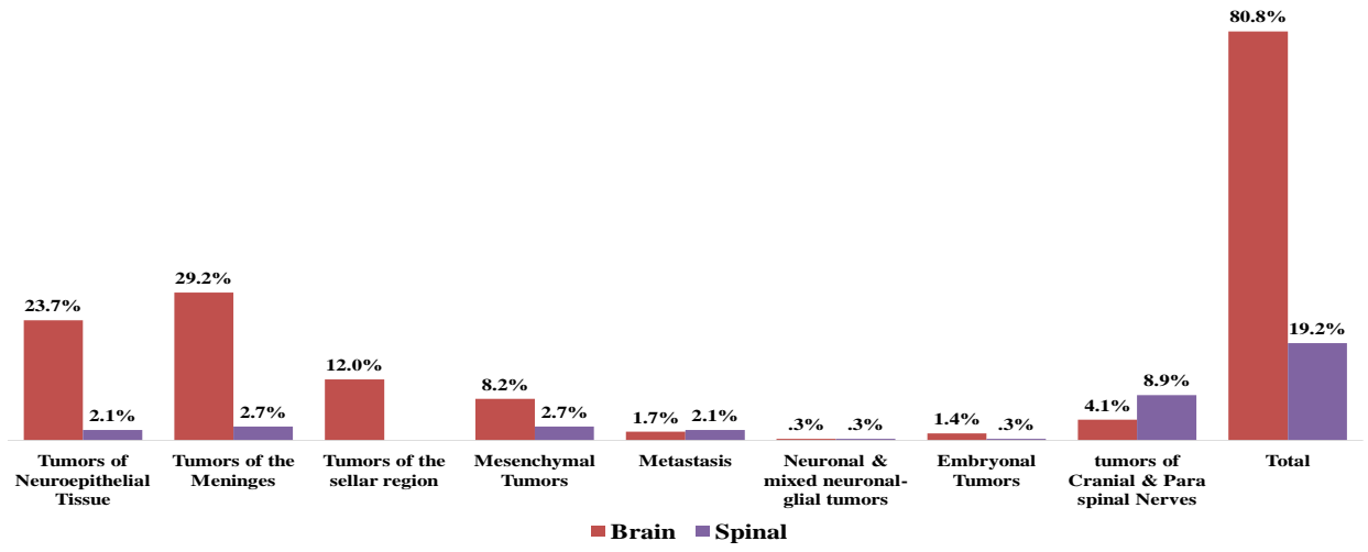
Fig. 10: Frequency of CNS Tumors among adult by site
