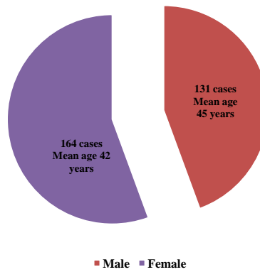
Fig 4: Adult age distribution in relation to sex n= 295 patients
