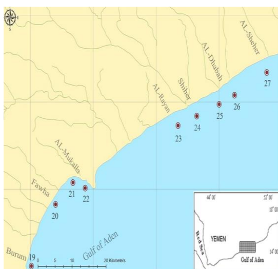
Figure 3: Sampling locations (19–27) along the Coast of AL-Mukalla city, Yemen.
