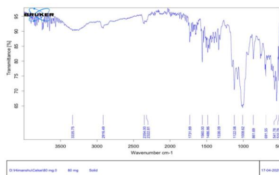
Figure 3: FT-IR result of 1:2, SLX:BCD inclusion complex.
