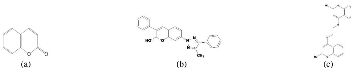
Figure 1: Structure of (a). Coumarin, (b). COU-130(7-(4-methyl-5-phenyl-2H-1,2,3-triazol-2-yl)-3-phenyl-2H-chromen-2-ol) (c). COU-220 (4-methoxy-2H-chromen-2-ol)
