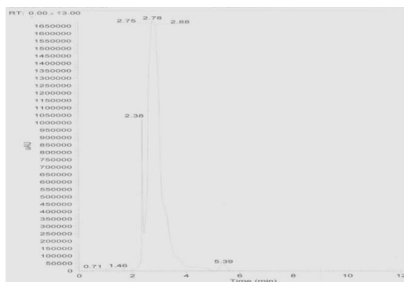
Figure 1: HPLC Spectrum of methanol extract of A. sinkatana leaf.
