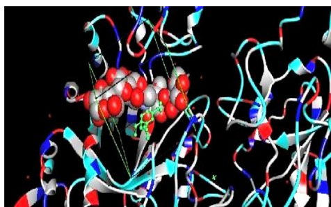
Figure 4: Isocaespitol.
