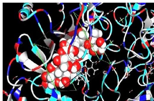
Figure 3: 1-ethenyl-1-methyl-2,4-di(prop-1-en-2-yl)cyclohexane.
