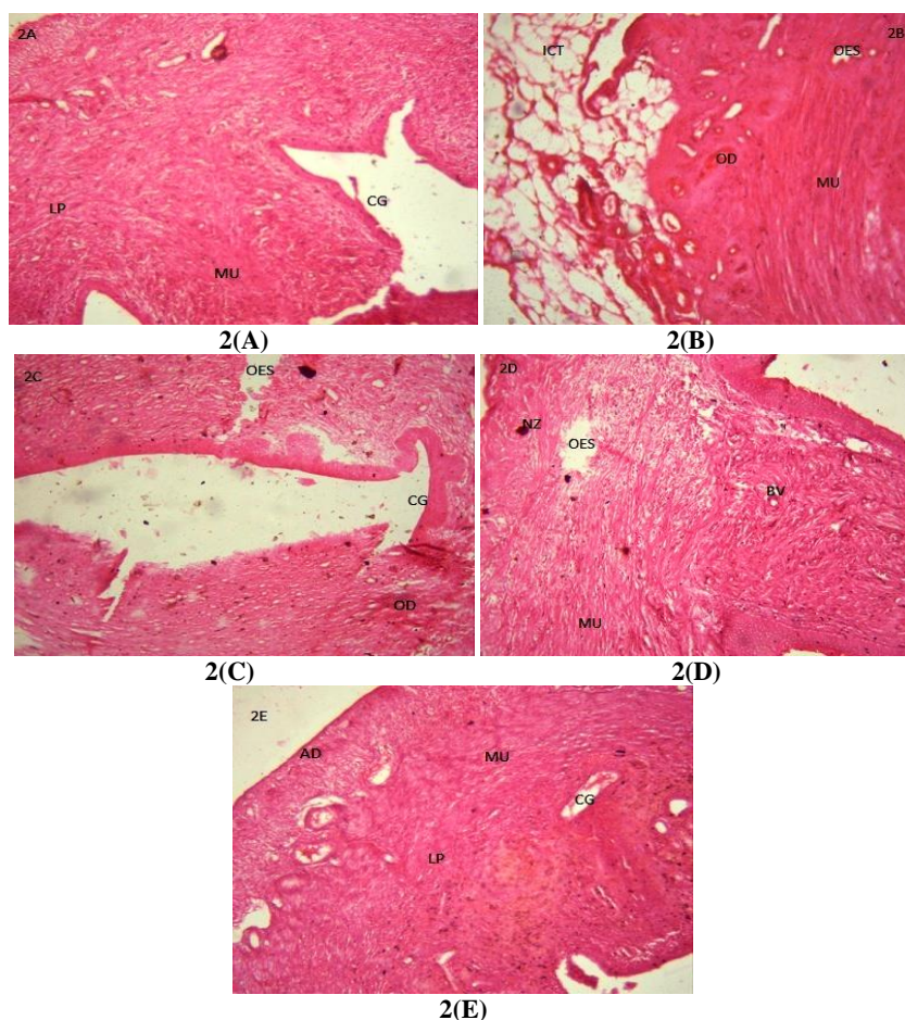
Figure: 2(A). The cervix of group A (negative control) revealed the presence of a normal mucosa, LP-Lamina propria and CG-Cervical gland. 2(B). Cervix following administration of lead acetate (1.5 mg/kg) for 14 days. OD-Oedema, FC-Fatty change, ICT-Interconnective tissue, MU-Muscle and OES-Optically Empty Space. H and E stains, 200X. 2(C). Cervix following administration of lead acetate (1.5 mg/kg) for 7 days and 24 hours later exposed to aqueous extract of F. vogelii (100 g/kg) for another 7 days. OD-Oedema, CG-Cervical gland and OES-Optically Empty Space. 2(D). Cervix following administration of lead acetate (1.5 mg/kg) for 7 days and 24 hours later exposed to aqueous extract of F. vogelii (300 g/kg) for another 7 days. OES-Optically Empty Space, MU-Muscle, NZ-Necrotic zone and Bv-Blood vessel. H and E stains, 200X. 2(E). Cervix following administration of aqueous extract of F. vogelii (300 g/kg) for another 14 days. MU-Muscle, CG-Cervical gland, LP-Lamina propria, and AD-adventitia. (H and E stains, 200X).
