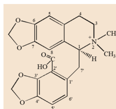
Figure 4: N-methylcoryximine.
